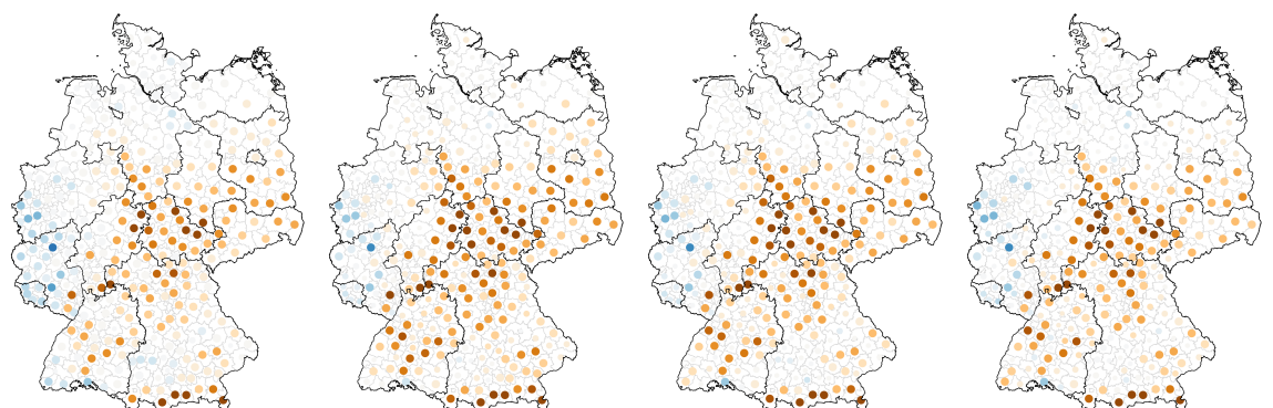
Fig. 3: Seasonal forecasts (2025-Dec to 2026-Jun); mean of total subsurface water storage anomalies from 50-member ParFlow/CLM ensemble (initialized on 2025-12-01), ECMWF SEAS seasonal ensemble prediction driven. Dots: NUTS-3 level administrative regions; dot size: proportional to how many members agree in their sign.
